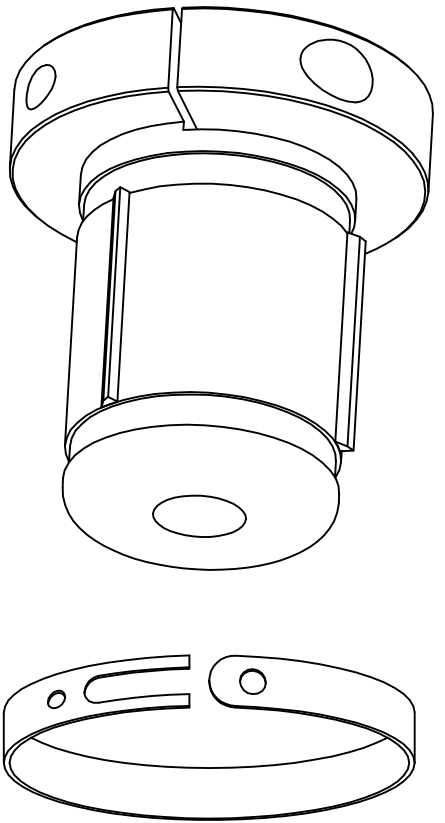
RETAINING BAND
